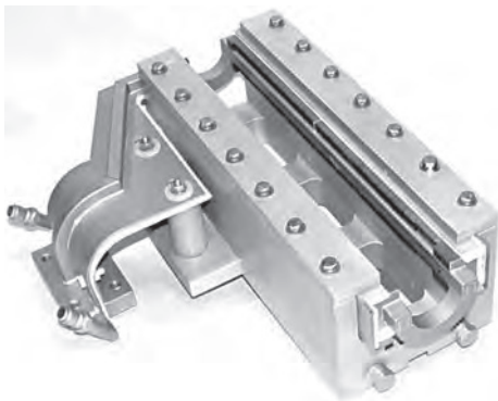
Fig. 3 Induction coil with laminations stacked between mechanical supports. Courtesy of Tucker Induction.
