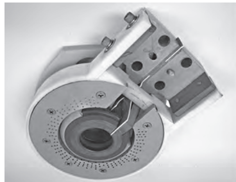
Fig. 27 Two-turn scan hardening coil with magnetic flux controllers used for axle scan hardening. Source: Ref 4
