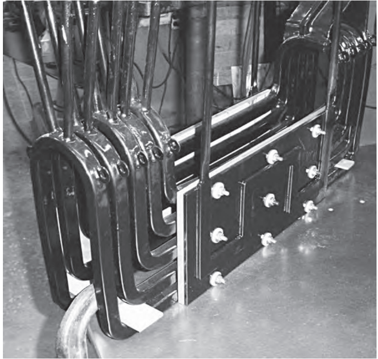
Fig. 20 Continuous bar-end heater with magnetic flux concentrator. Courtesy of Fluxtrol, Inc.
