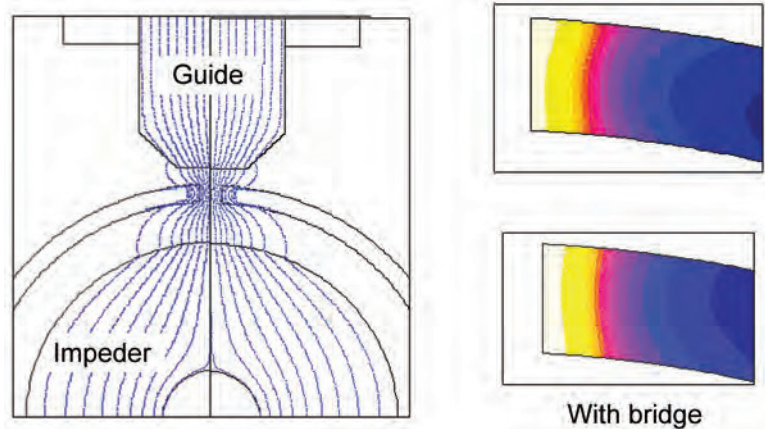
Fig. 24 Influence of a magnetic bridge on weld temperature distribution for a 40 mm OD by 2.5 mm thick tube traveling at a line velocity of 75 m/min; the bridge helps balance heating of the top and bottom edges of the tube wall. Source: Ref 4
